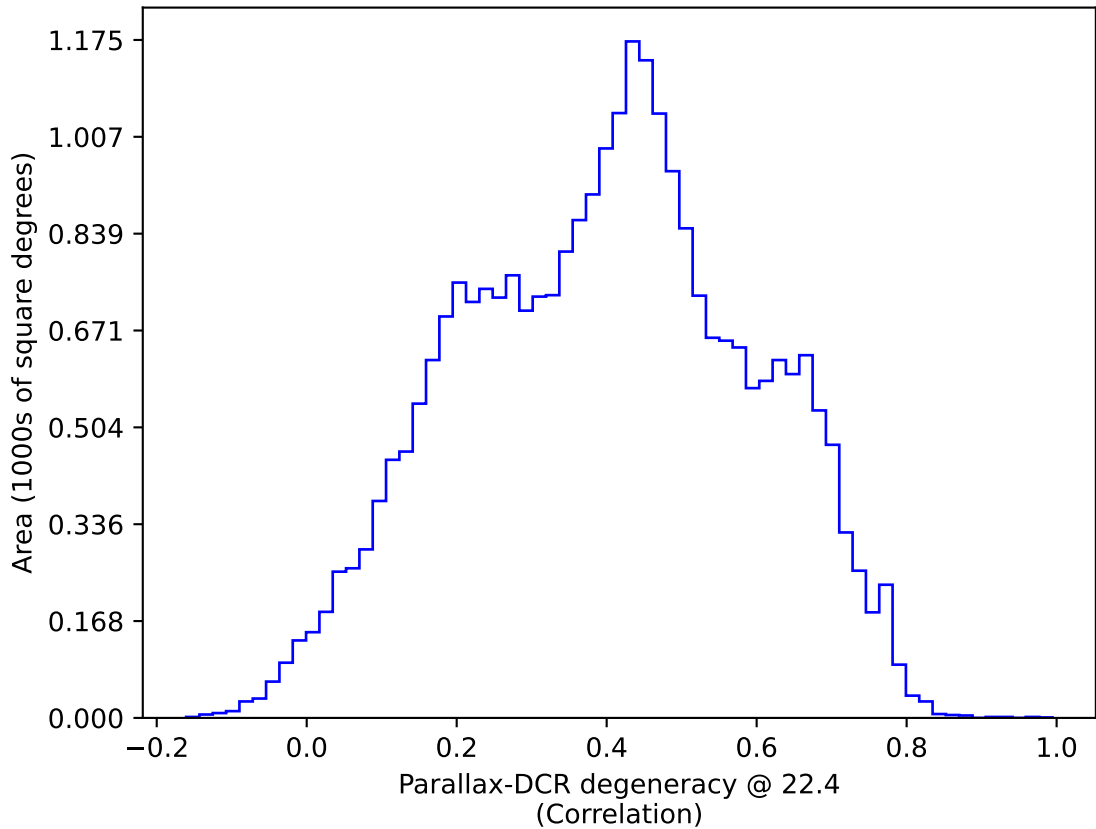
weather_cloudso35v3.4_10yrs : Parallax-DCR degeneracy @ 22.4
