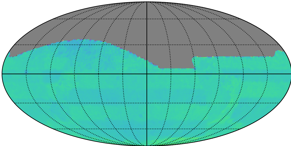
weather_cloudso35v3.4_10yrs : Normalized Proper Motion Uncert @ 20.5
