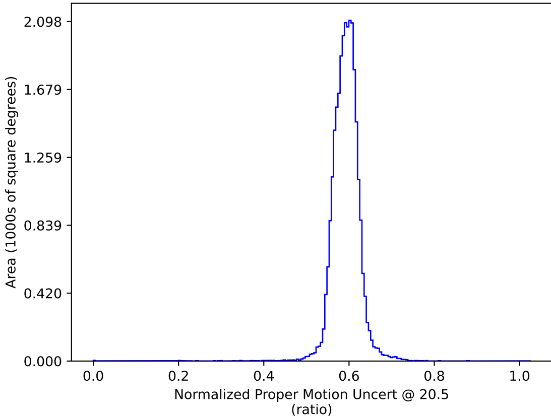
weather_cloudso35v3.4_10yrs : Normalized Proper Motion Uncert @ 20.5
