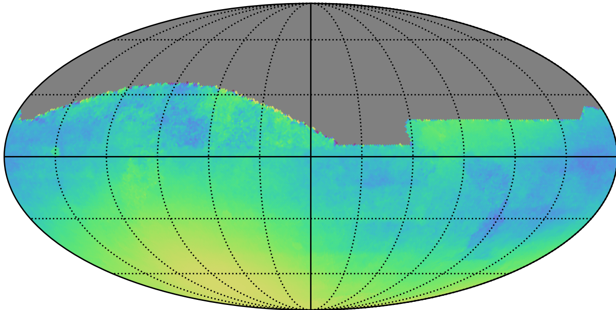
weather_cloudso35v3.4_10yrs : Normalized Parallax Uncert @ 22.4
