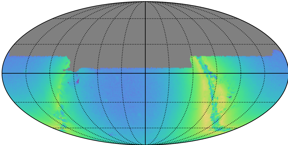
weather_cloudso35v3.4_10yrs u: N stars to Precision 0.20
