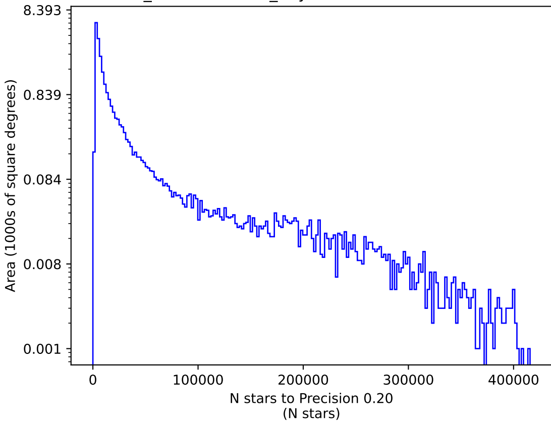
weather_cloudso35v3.4_10yrs u: N stars to Precision 0.20
