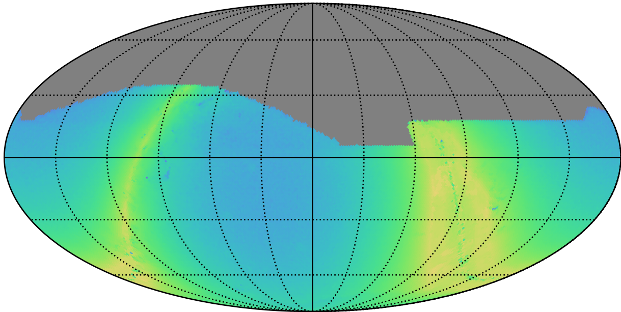
weather_cloudso35v3.4_10yrs r: N stars to Precision 0.20
