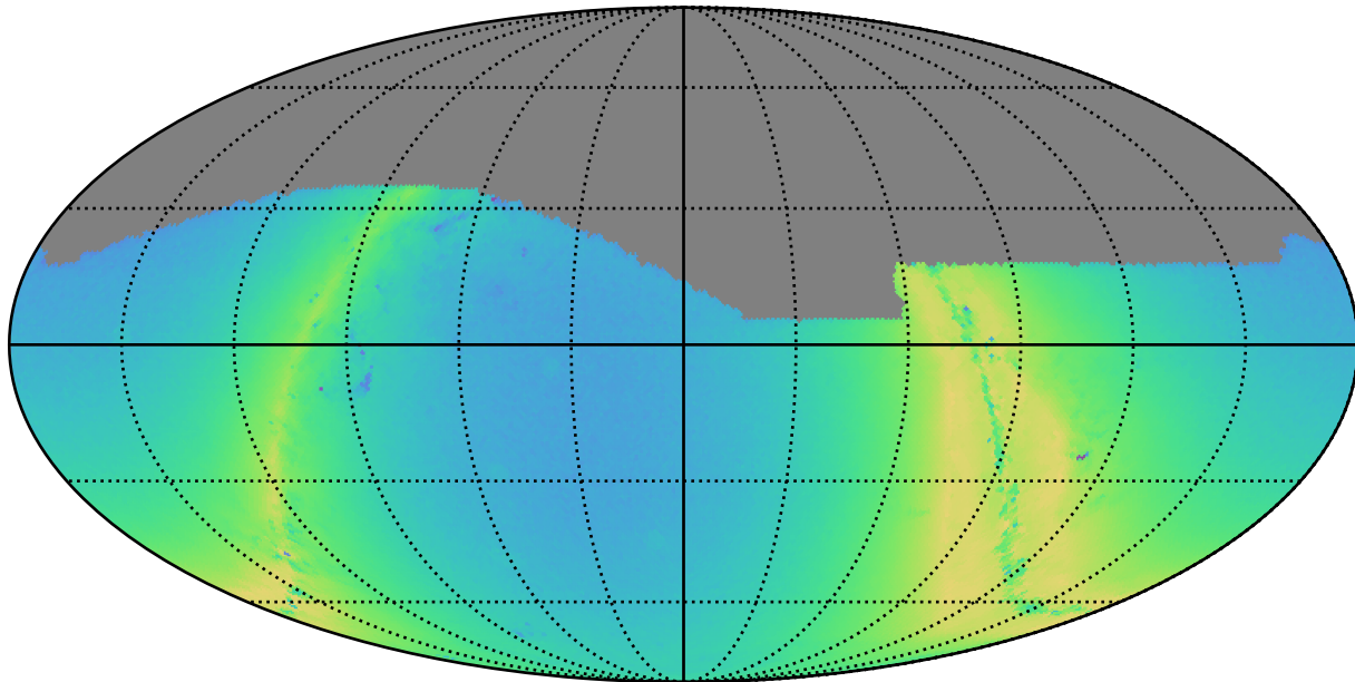
weather_cloudso35v3.4_10yrs g: N stars to Precision 0.20
