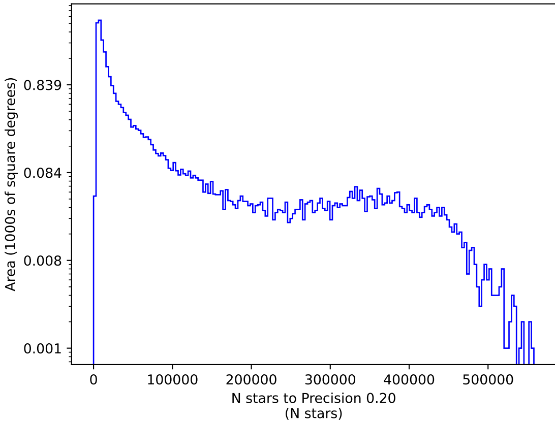
weather_cloudso35v3.4_10yrs g: N stars to Precision 0.20
