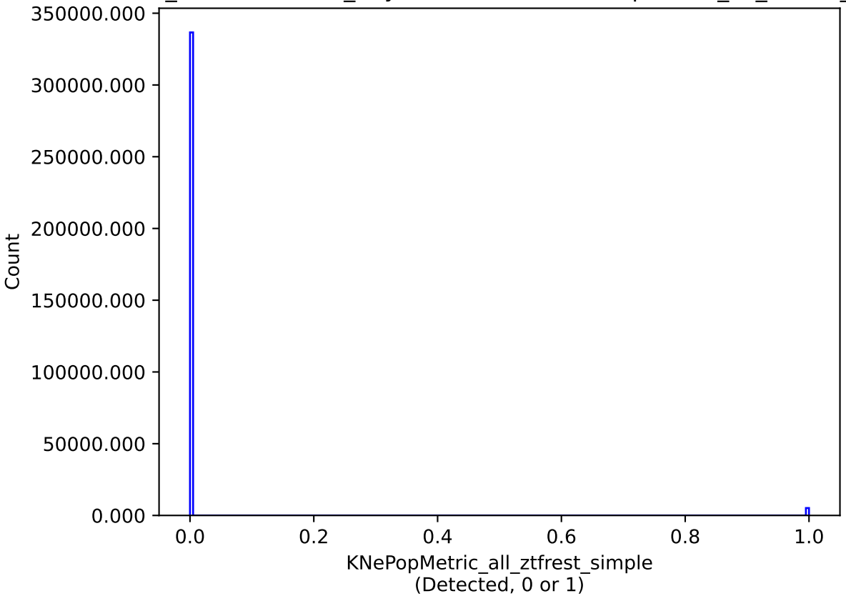
weather_cloudso35v3.4_10yrs all models: KNePopMetric_all_ztfrest_simple
