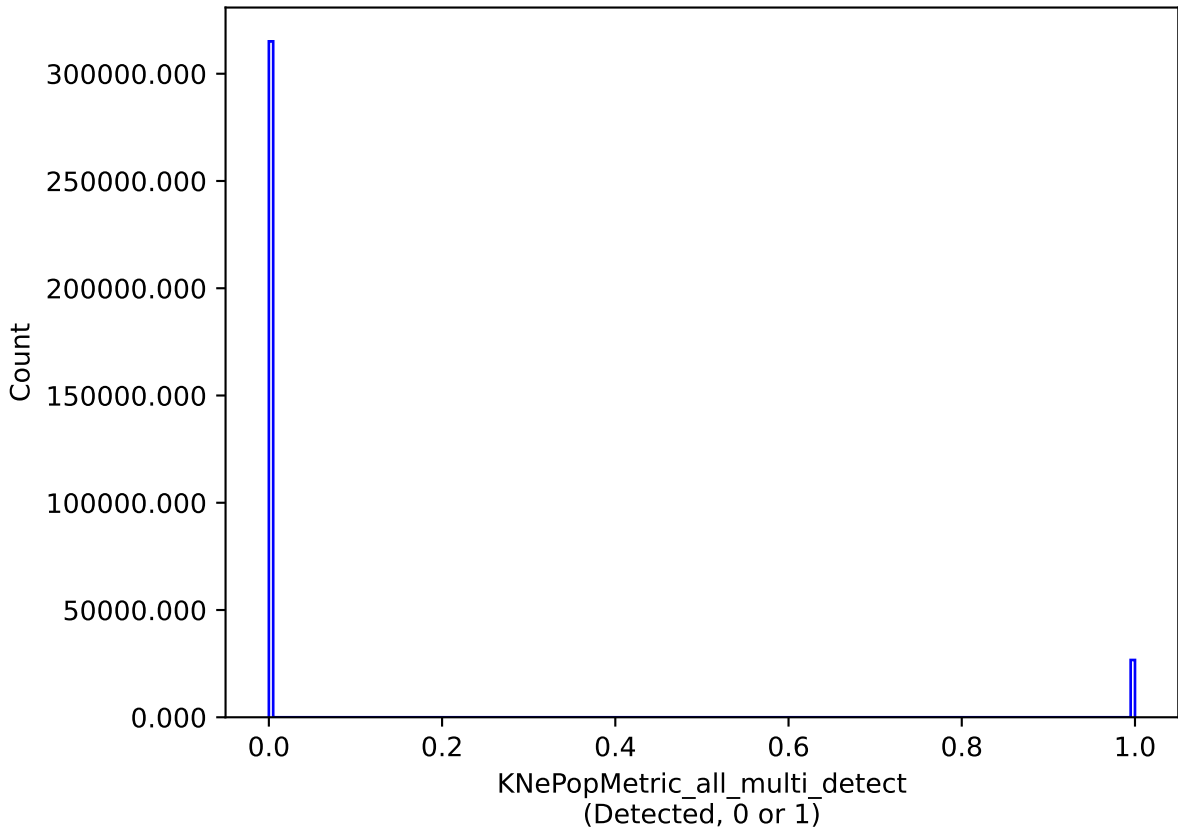
weather_cloudso35v3.4_10yrs all models: KNePopMetric_all_multi_detect
