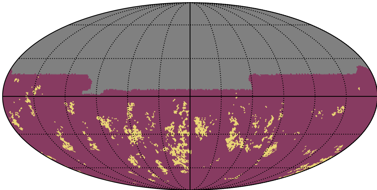
weather_cloudso35v3.4_10yrs u band: Gaps_7hr
