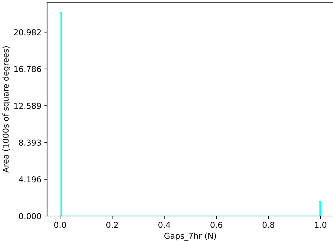
weather_cloudso35v3.4_10yrs u band: Gaps_7hr
