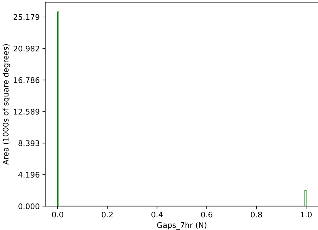
weather_cloudso35v3.4_10yrs g band: Gaps_7hr
