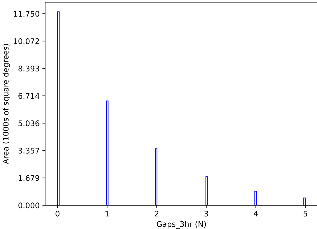
weather_cloudso35v3.4_10yrs y band: Gaps_3hr
