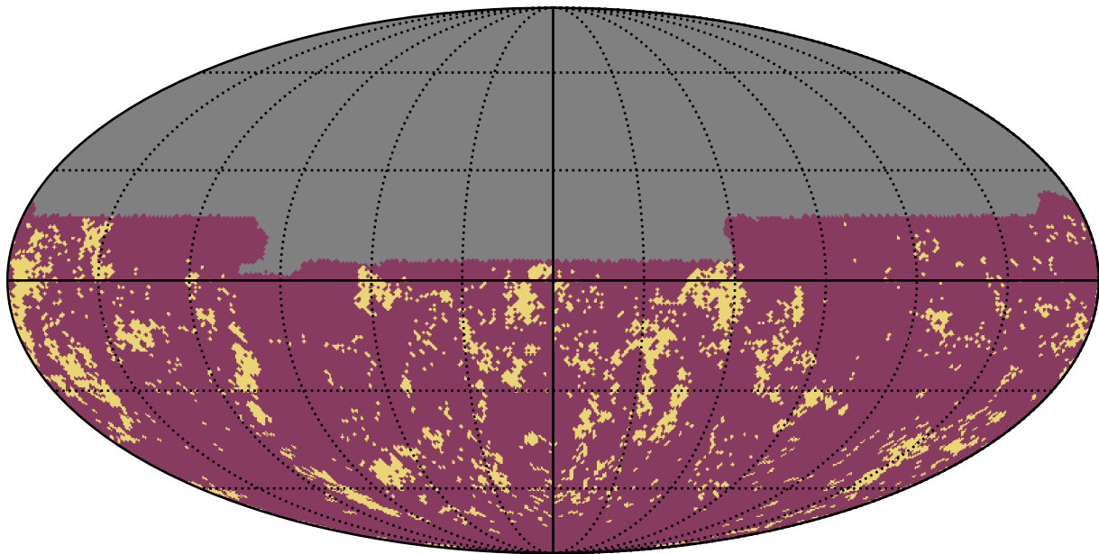
weather_cloudso35v3.4_10yrs u band: Gaps_3hr
