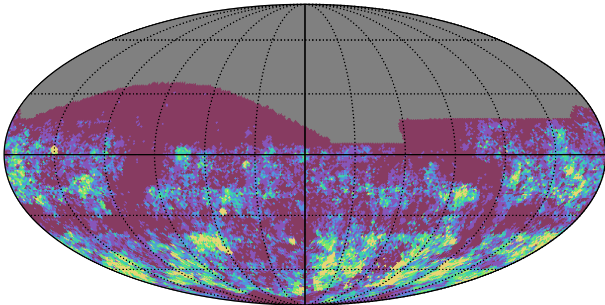
weather_cloudso35v3.4_10yrs r band: Gaps_3hr
