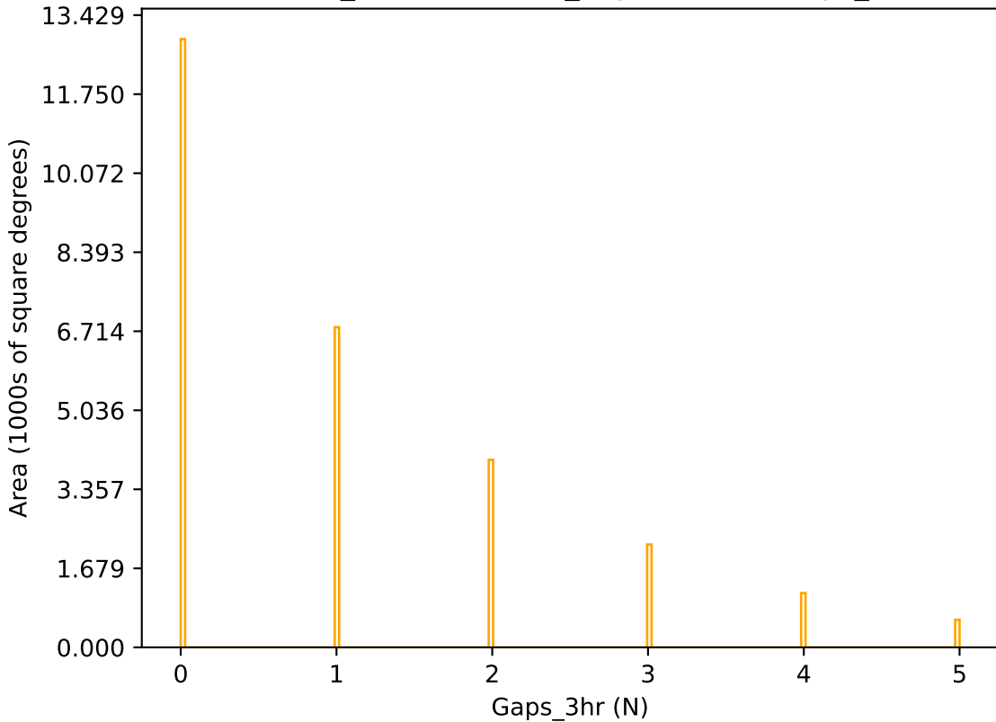
weather_cloudso35v3.4_10yrs r band: Gaps_3hr
