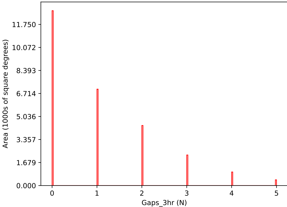
weather_cloudso35v3.4_10yrs i band: Gaps_3hr
