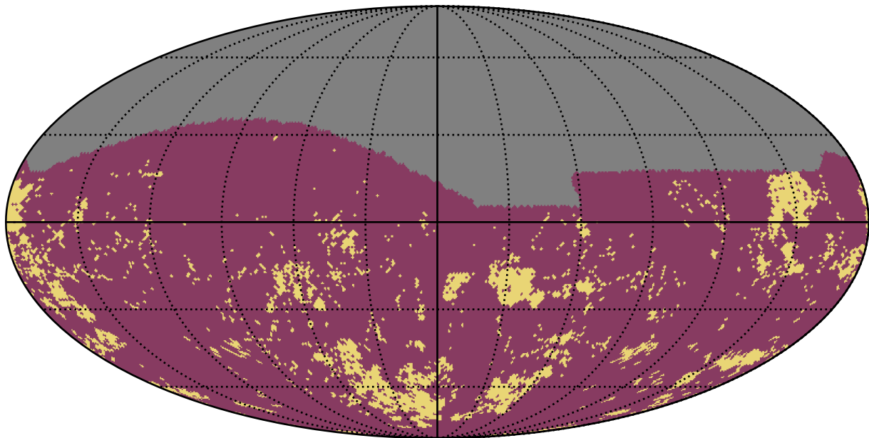
weather_cloudso35v3.4_10yrs g band: Gaps_3hr
