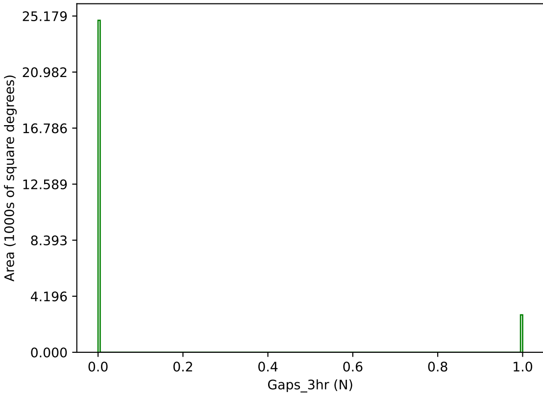
weather_cloudso35v3.4_10yrs g band: Gaps_3hr
