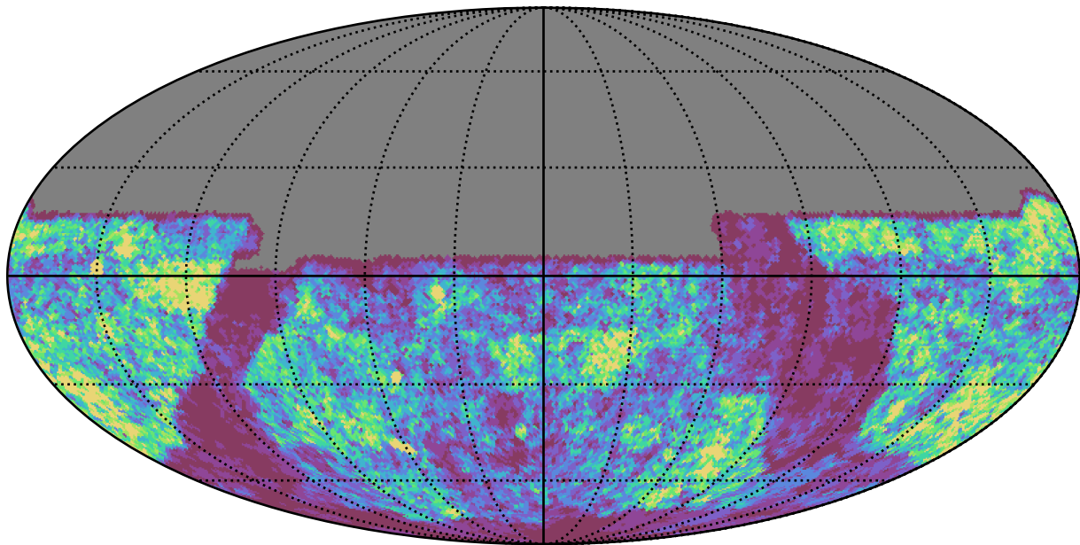
weather_cloudso35v3.4_10yrs u band: Gaps_24hr
