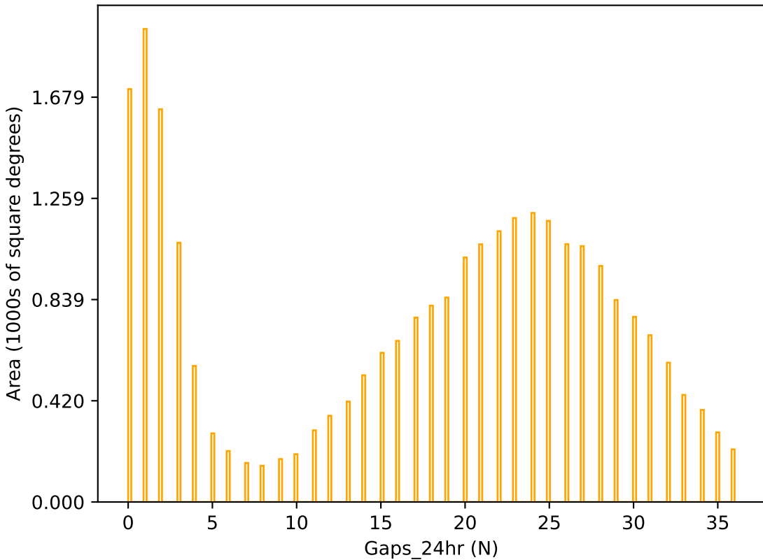
weather_cloudso35v3.4_10yrs r band: Gaps_24hr
