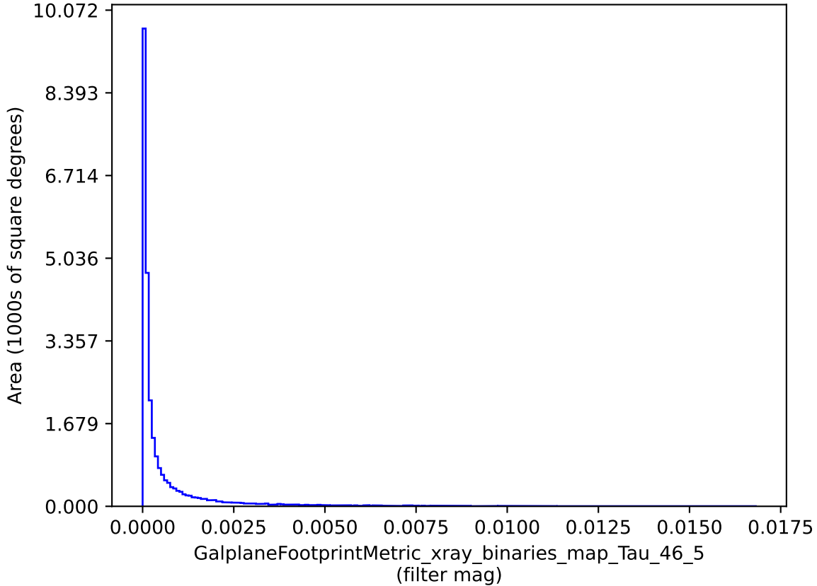
weather_cloudso35v3.4_10yrs : GalplaneFootprintMetric_xray_binaries_map_Tau_46_5
