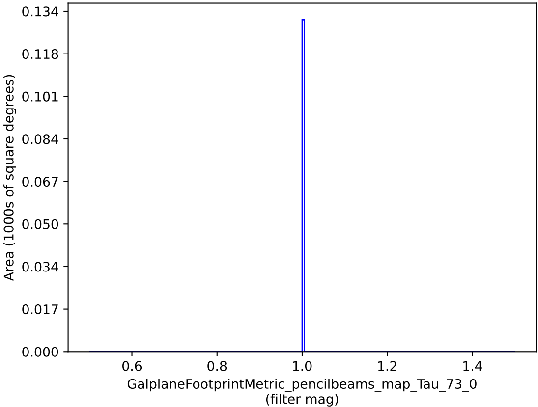
weather_cloudso35v3.4_10yrs : GalplaneFootprintMetric_pencilbeams_map_Tau_73_0
