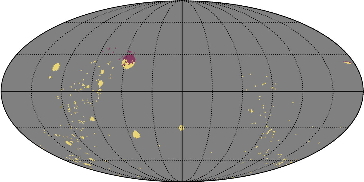
weather_cloudso35v3.4_10yrs : GalplaneFootprintMetric_open_clusters_map_Tau_73_0
