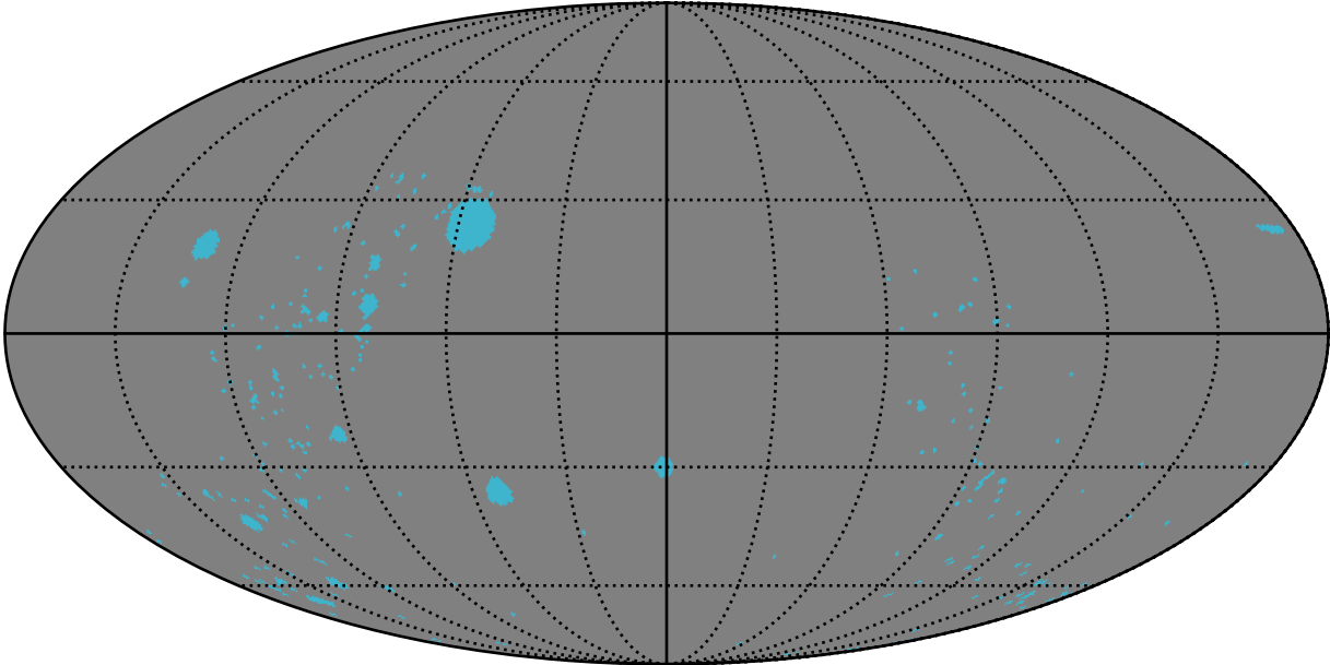
weather_cloudso35v3.4_10yrs : GalplaneFootprintMetric_open_clusters_map_Tau_2_0
