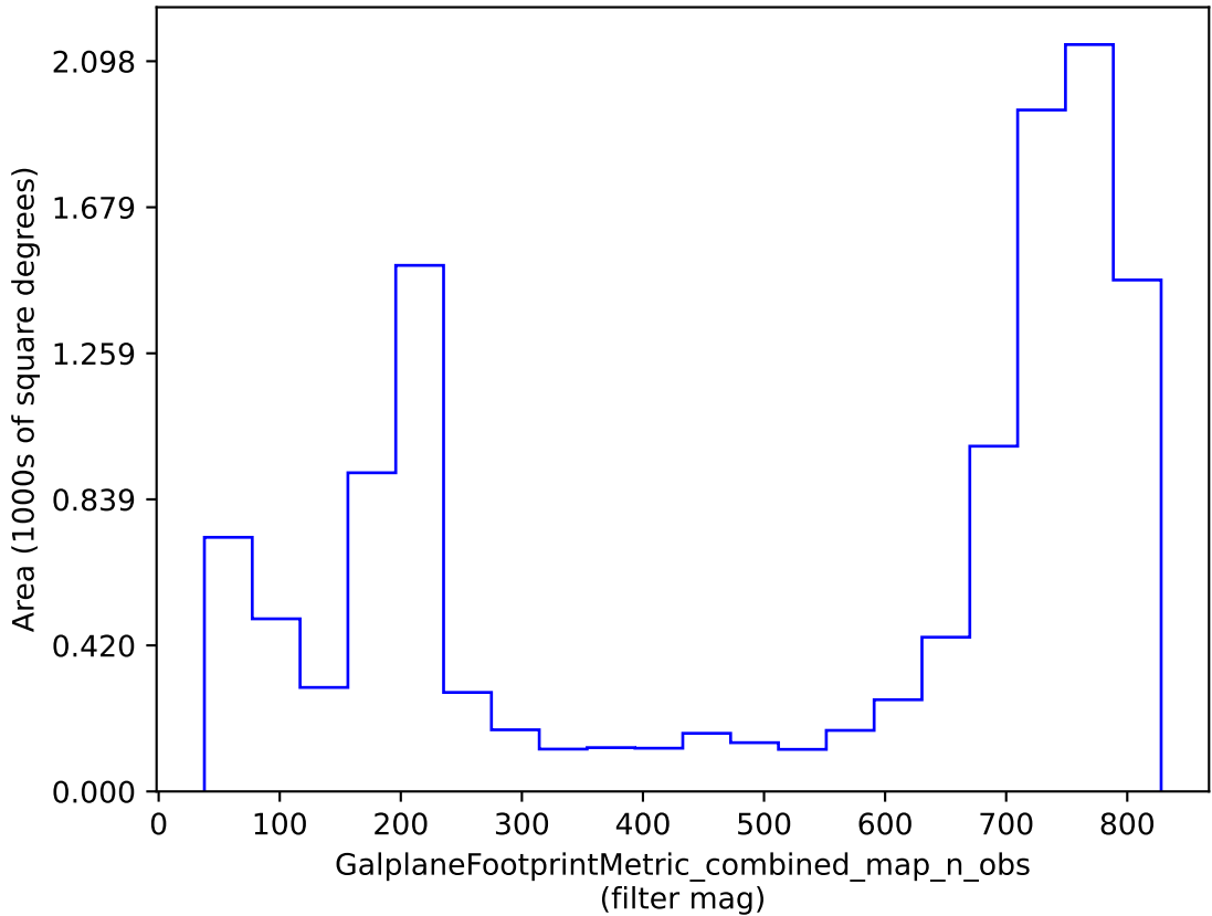
weather_cloudso35v3.4_10yrs : GalplaneFootprintMetric_combined_map_n_obs
