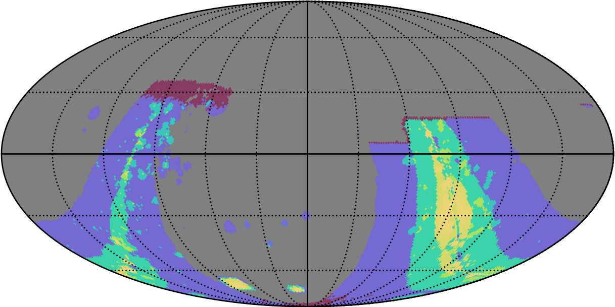
weather_cloudso35v3.4_10yrs : GalplaneFootprintMetric_combined_map_Tau_73_0
