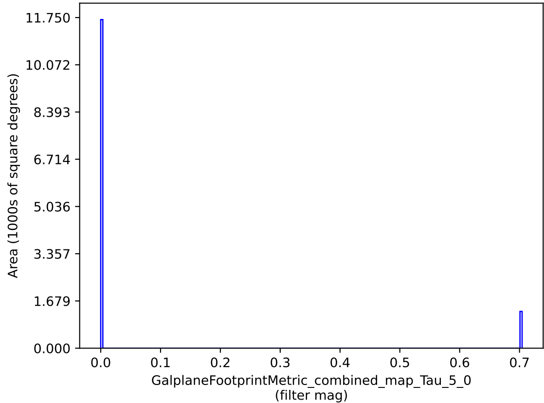
weather_cloudso35v3.4_10yrs : GalplaneFootprintMetric_combined_map_Tau_5_0
