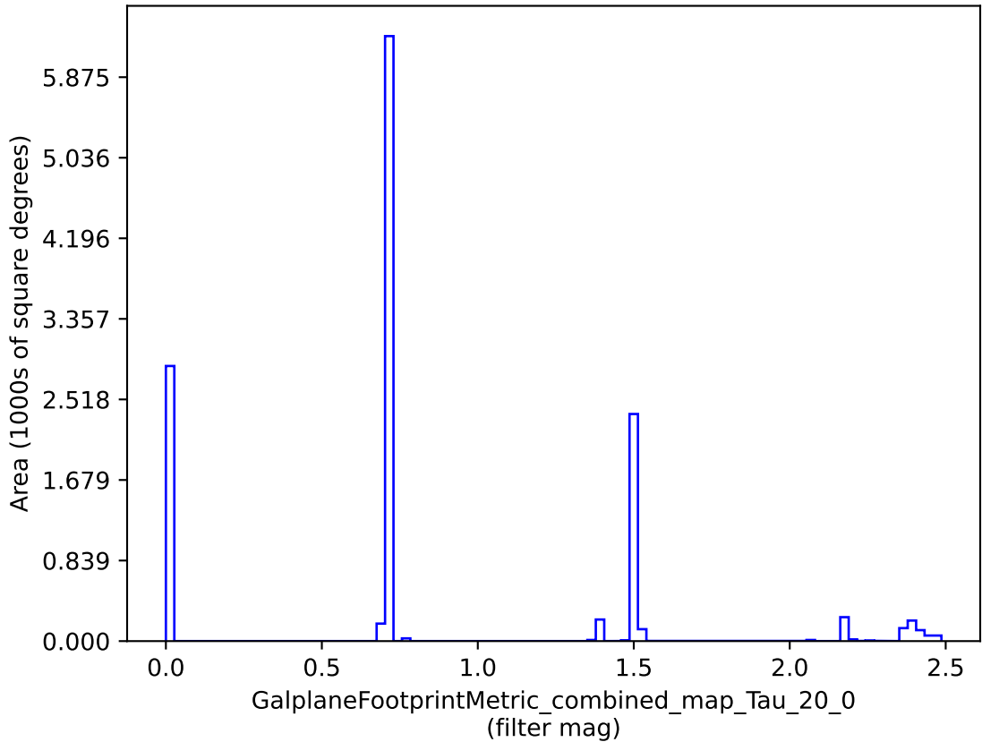
weather_cloudso35v3.4_10yrs : GalplaneFootprintMetric_combined_map_Tau_20_0
