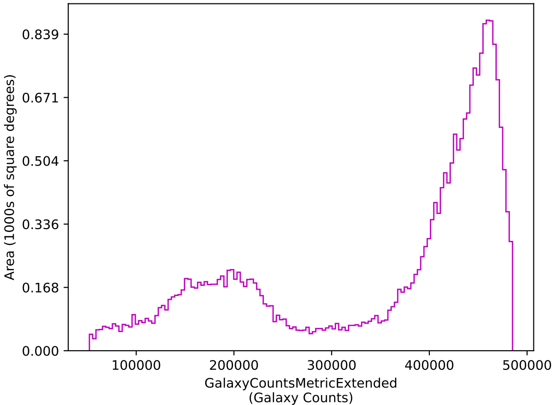
weather_cloudso35v3.4_10yrs z: GalaxyCountsMetricExtended
