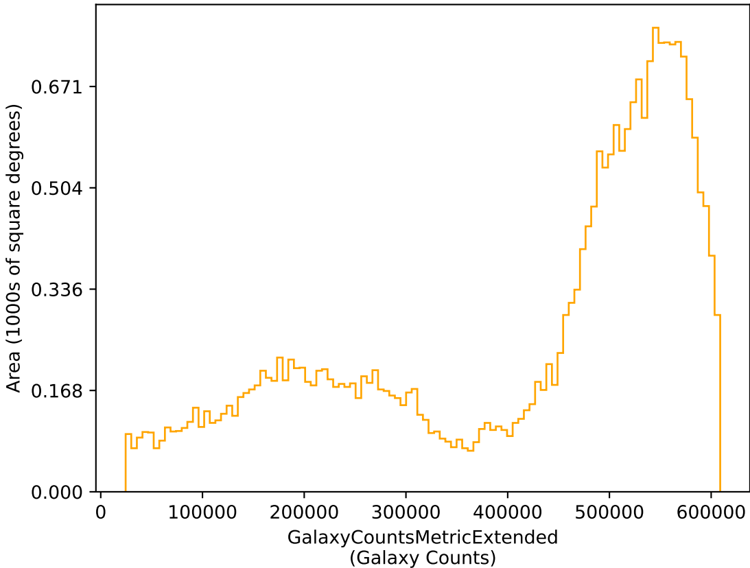
weather_cloudso35v3.4_10yrs r: GalaxyCountsMetricExtended
