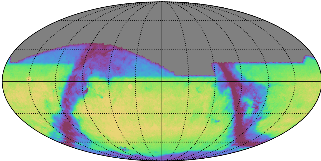
weather_cloudso35v3.4_10yrs i: GalaxyCountsMetricExtended
