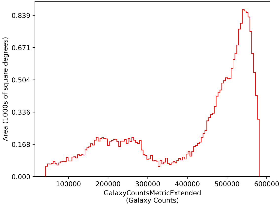
weather_cloudso35v3.4_10yrs i: GalaxyCountsMetricExtended
