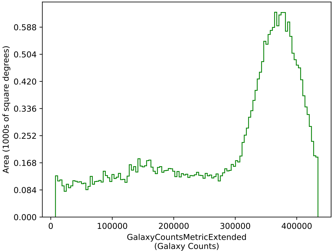
weather_cloudso35v3.4_10yrs g: GalaxyCountsMetricExtended
