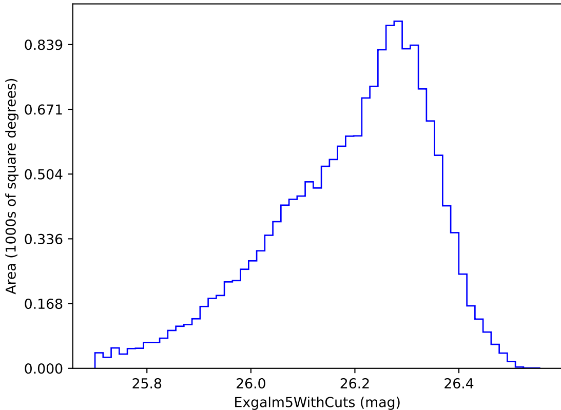
weather_cloudso35v3.4_10yrs i band non-DD year 7: ExgalM5WithCuts
