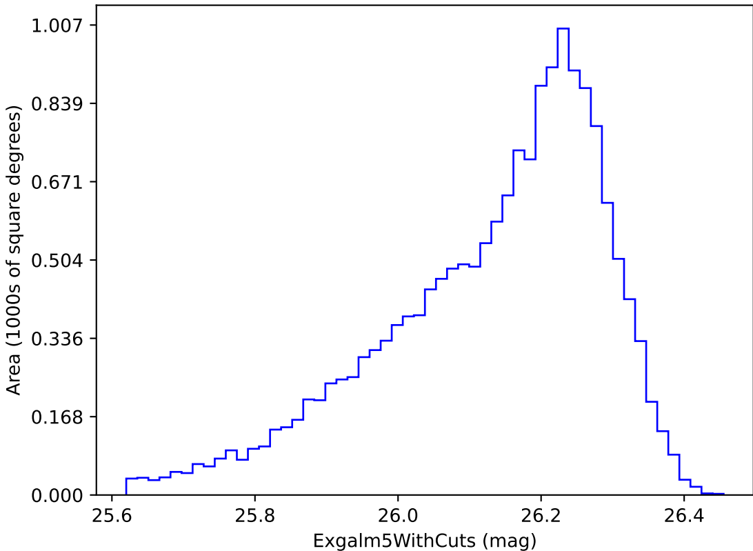
weather_cloudso35v3.4_10yrs i band non-DD year 6: ExgalM5WithCuts
