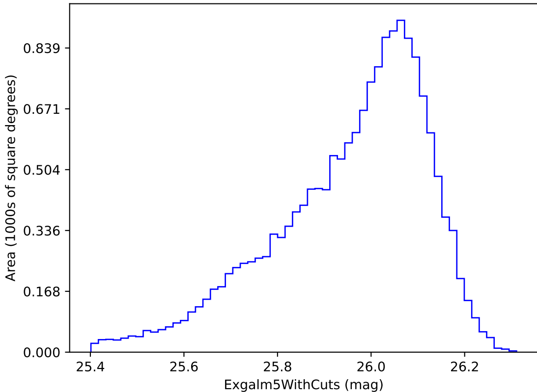
weather_cloudso35v3.4_10yrs i band non-DD year 4: ExgalM5WithCuts
