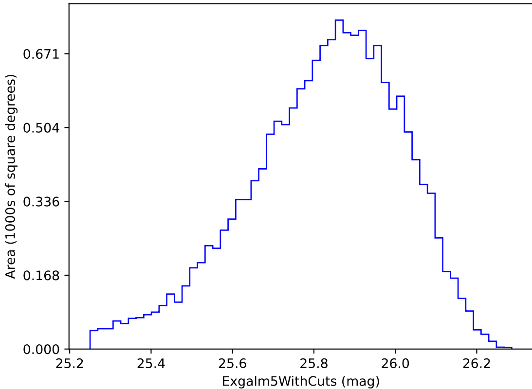
weather_cloudso35v3.4_10yrs i band non-DD year 3: ExgalM5WithCuts
