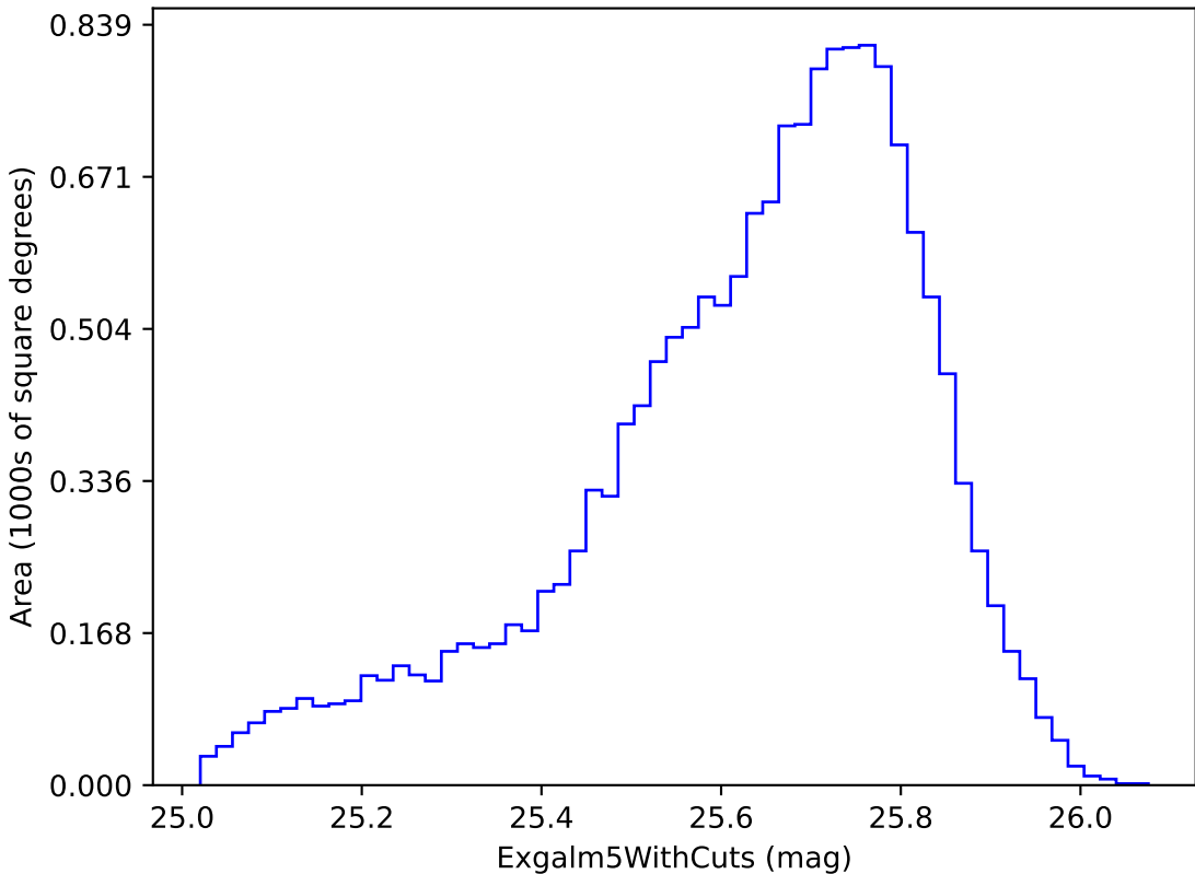
weather_cloudso35v3.4_10yrs i band non-DD year 2: ExgalM5WithCuts
