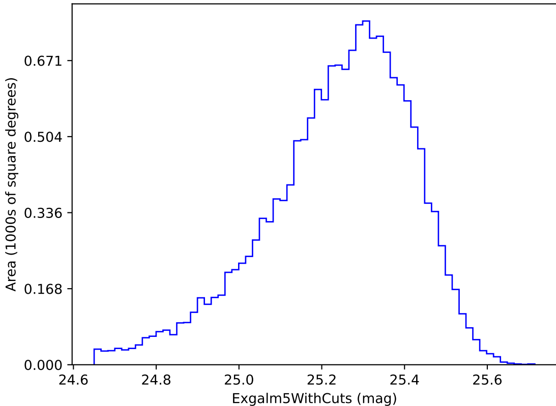
weather_cloudso35v3.4_10yrs i band non-DD year 1: ExgalM5WithCuts
