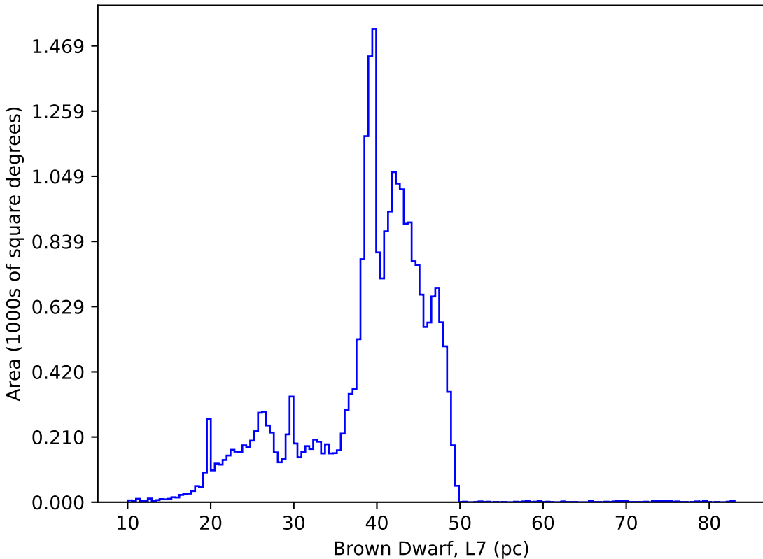
weather_cloudso35v3.4_10yrs : Brown Dwarf, L7
