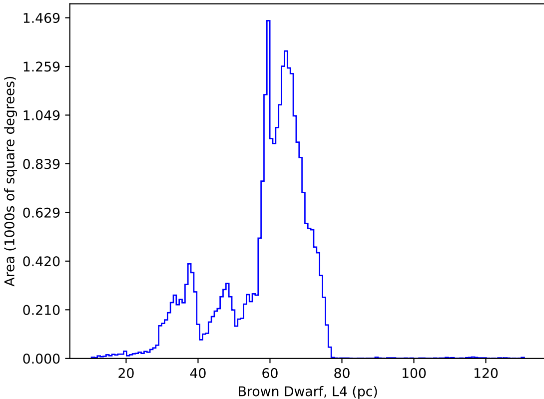
weather_cloudso35v3.4_10yrs : Brown Dwarf, L4
