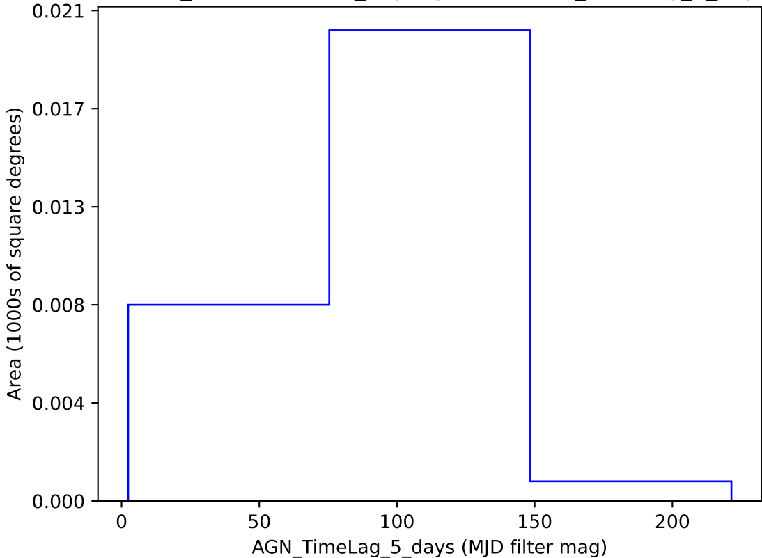
weather_cloudso35v3.4_10yrs y band: AGN_TimeLag_5_days
