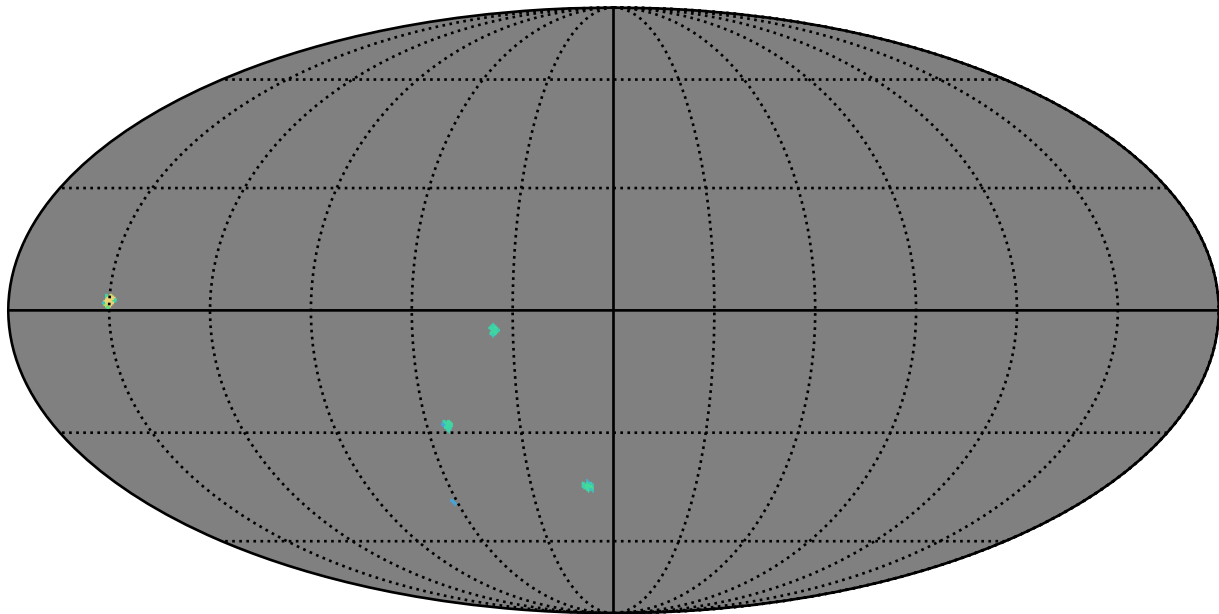
weather_cloudso35v3.4_10yrs r band: AGN_TimeLag_5_days
