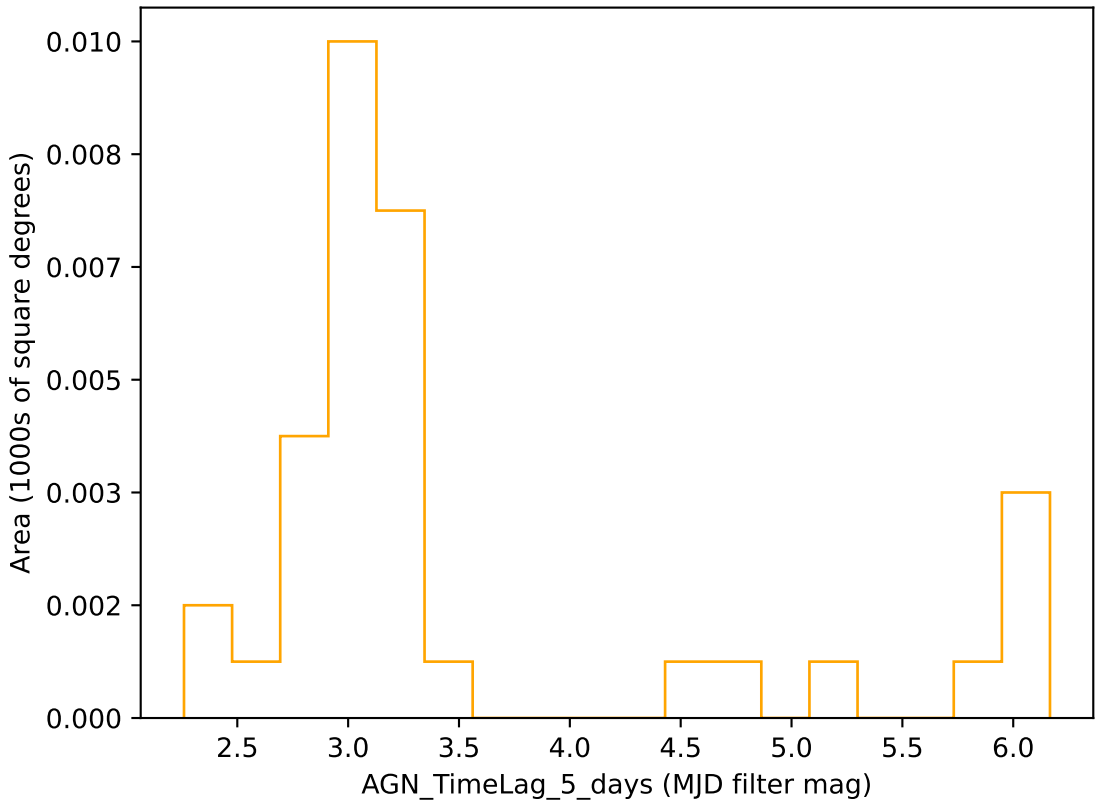
weather_cloudso35v3.4_10yrs r band: AGN_TimeLag_5_days
