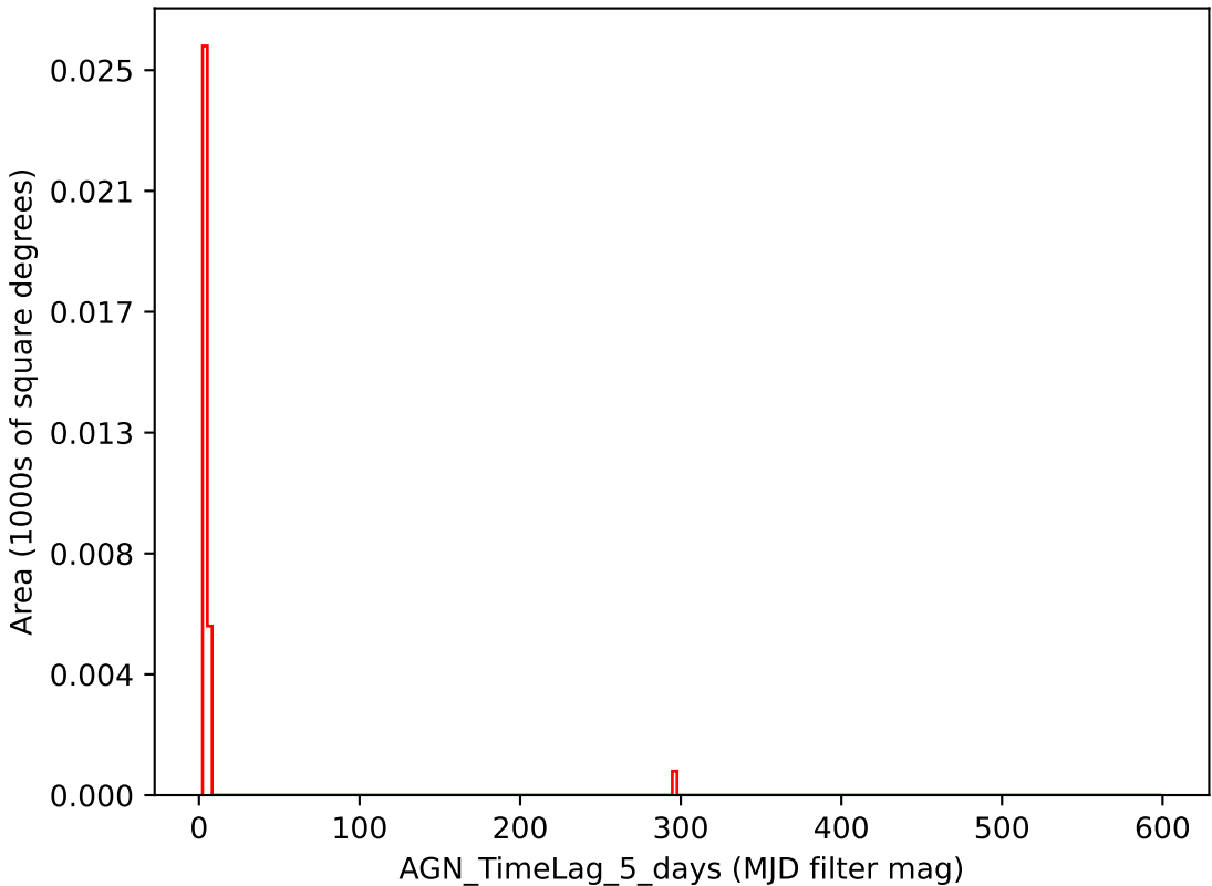
weather_cloudso35v3.4_10yrs i band: AGN_TimeLag_5_days
