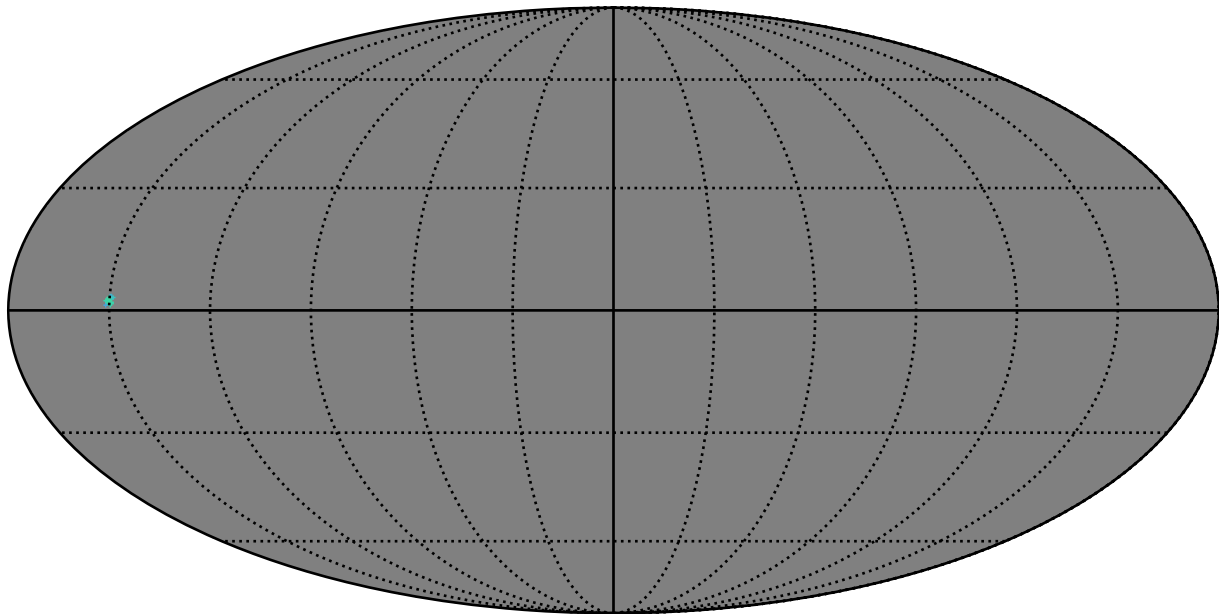
weather_cloudso35v3.4_10yrs g band: AGN_TimeLag_5_days
