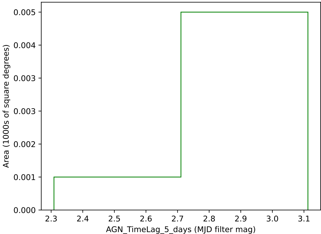
weather_cloudso35v3.4_10yrs g band: AGN_TimeLag_5_days
